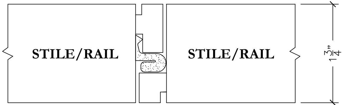
SHIPLAP DETAIL #2
