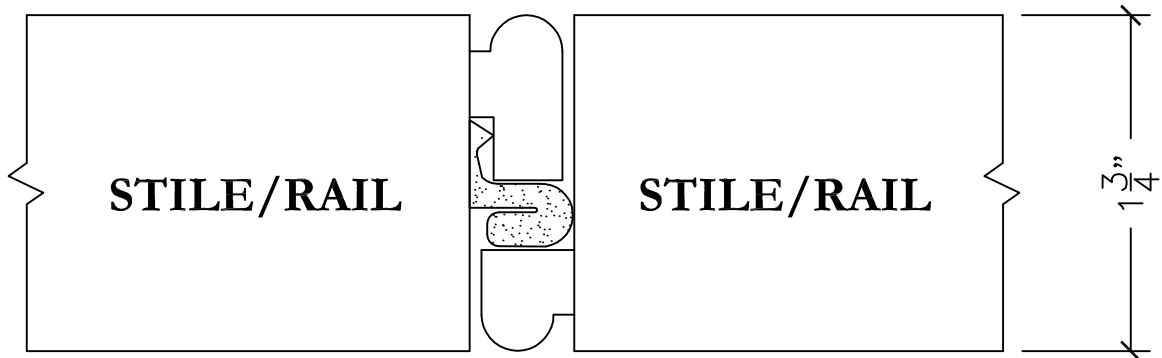
SHIPLAP DETAIL #1
