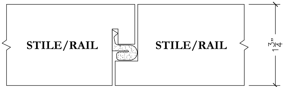
HALFLAP DETAIL
