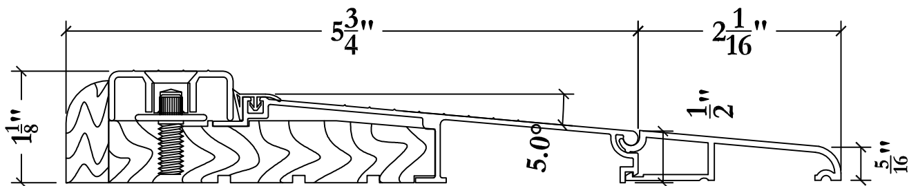
ALUMINUM SILL W/ADJUSTABLE OAK STRIP SHOWN WITH OPTIONAL EXTENSION
