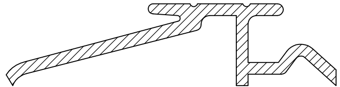
#842 INTERLOCK SADDLE (VARIOUS FINISHES AVAILABLE) IN SWING ONLY
