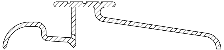
#145 INTERLOCK SADDLE (VARIOUS FINISHES AVAILABLE) IN SWING ONLY
