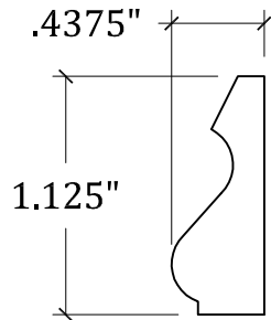
APPLIED MOLDING - A101
