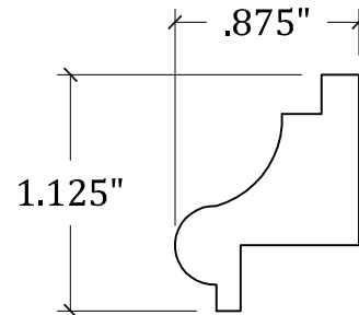
RAISED MOLDING - R102
