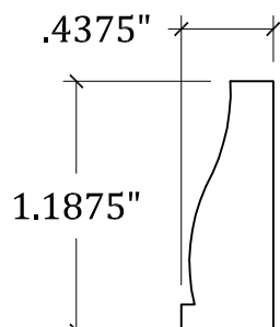
APPLIED MOLDING - A103
