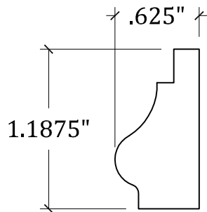
APPLIED MOLDING - A102
