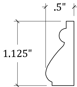
APPLIED MOLDING - A103
