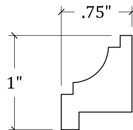
RAISED MOLDING - R103
