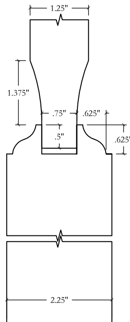
DETAIL: STILE @ PANEL COPE - OGEE S01 PANEL - SCOOPED P01
