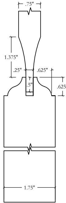
DETAIL: STILE @ PANEL COPE - OGEE S01 PANEL - SCOOPED P01
