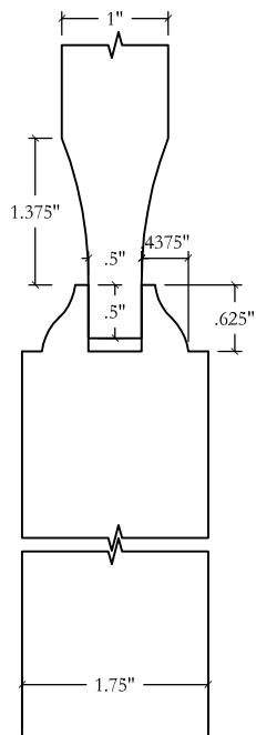
DETAIL: STILE @ PANEL COPE - OGEE S01 PANEL - SCOOPED P01
