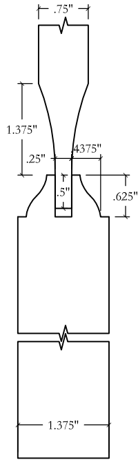
DETAIL: STILE @ PANEL COPE - OGEE S01 PANEL - SCOOPED P01
