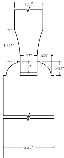
DETAIL: STILE @ GLASS COPE - OVOLO S02 PANEL - SCOOPED P01
