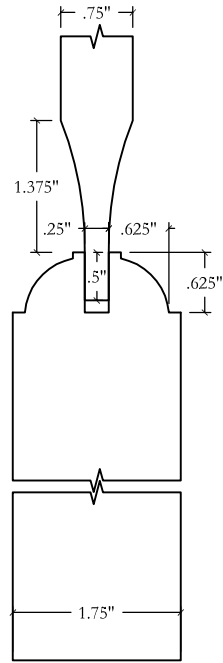
DETAIL: STILE @ GLASS COPE - OVOLO S02 PANEL - SCOOPED P01
