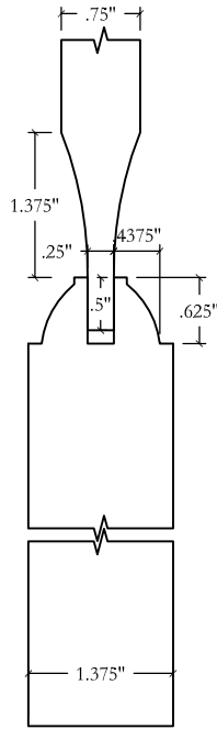
DETAIL: STILE @ GLASS COPE - OVOLO S02 PANEL - SCOOPED P01
