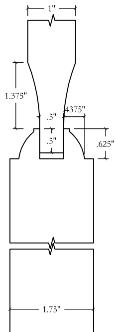
DETAIL: STILE @ GLASS COPE - OVOLO S02 PANEL - SCOOPED P01
