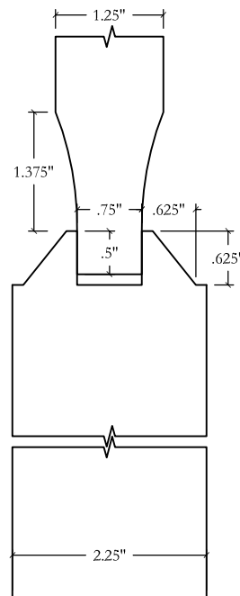
DETAIL: STILE @ GLASS COPE - BEVEL S04 PANEL - SCOOPED P01
