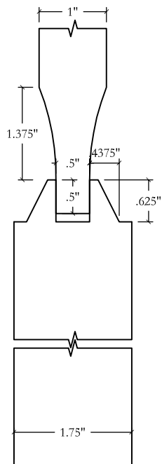
DETAIL: STILE @ PANEL COPE - BEVEL S04 PANEL - SCOOPED P01
