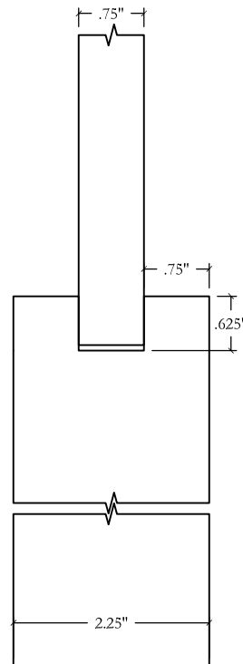
DETAIL: STILE @ PANEL COPE - SQUARE S05 PANEL - FLAT P02
