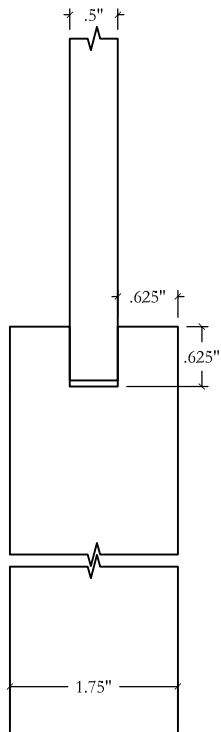
DETAIL: STILE @ PANEL COPE - SQUARE S05 PANEL - FLAT P02
