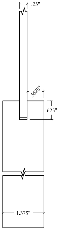
DETAIL: STILE @ PANEL COPE - SQUARE S05 PANEL - FLAT P02
