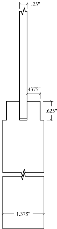
DETAIL: STILE @ PANEL COPE - SQUARE with STEP S06 PANEL - FLAT P02
