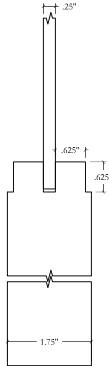
DETAIL: STILE @ PANEL COPE - SQUARE with STEP S06 PANEL - FLAT P02
