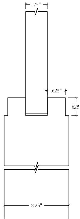
DETAIL: STILE @ PANEL COPE - SQUARE with STEP S06 PANEL - FLAT P02
